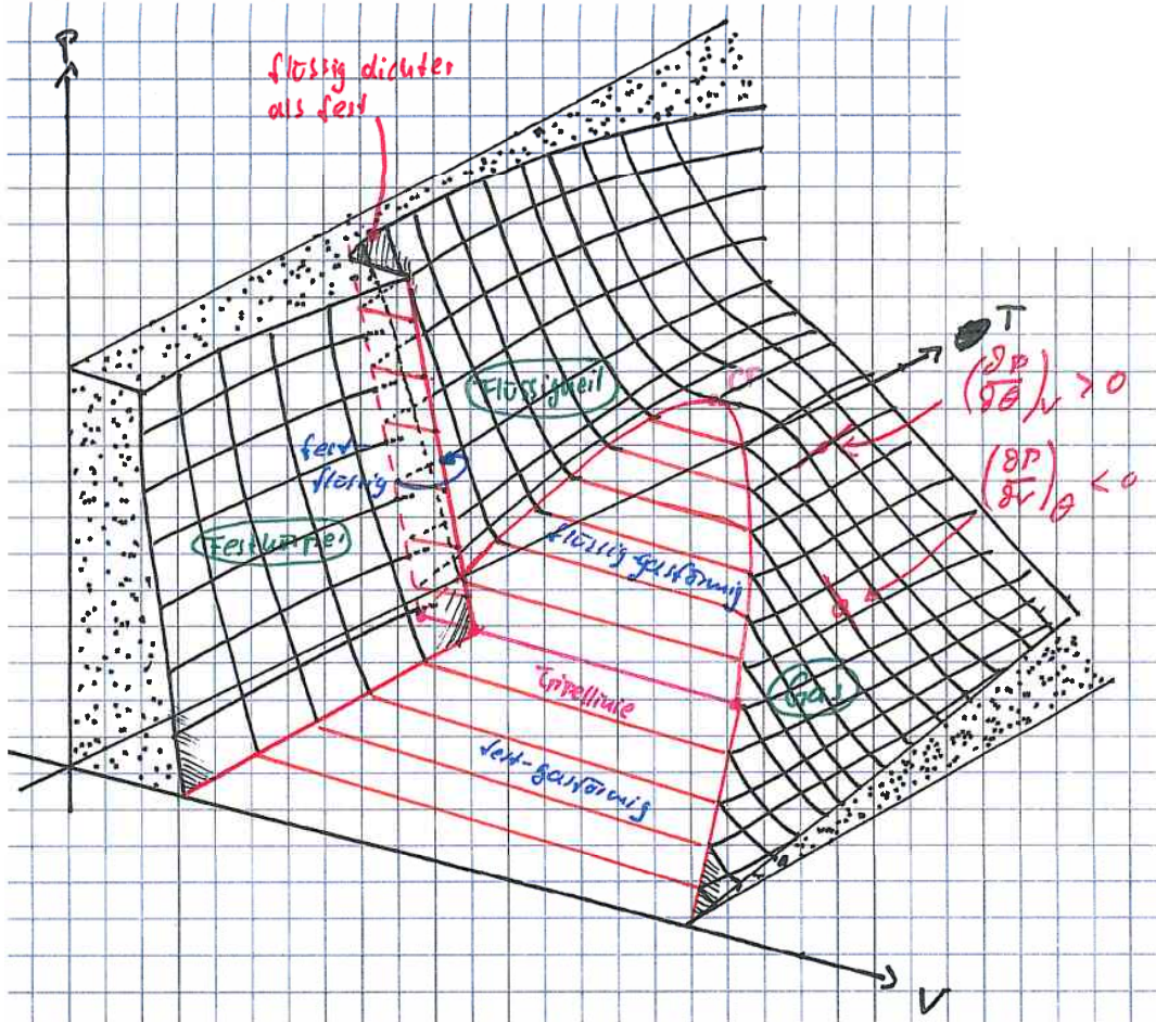
V-T-P diagram
