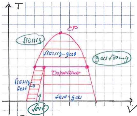
V-T diagram
