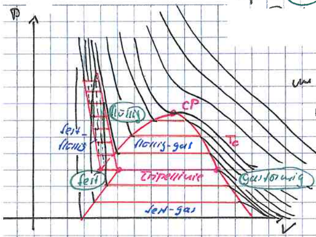
V-P diagram
